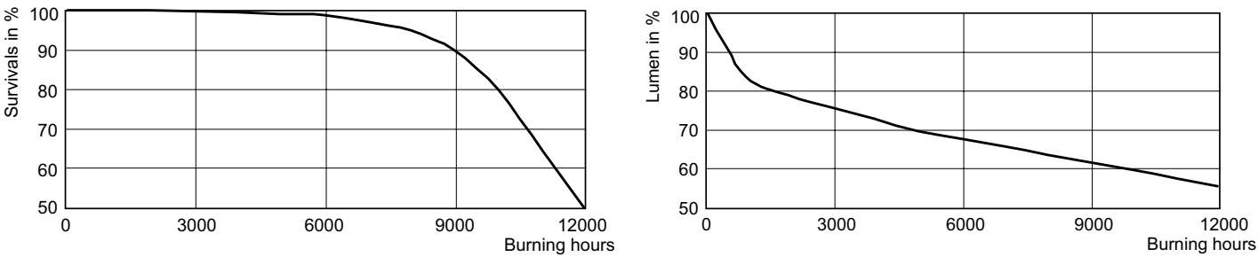
CDM-Tm Elite 20W Life Expectancy /830 PGJ5
