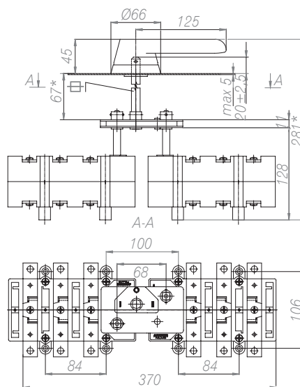
160 A – 250 A
