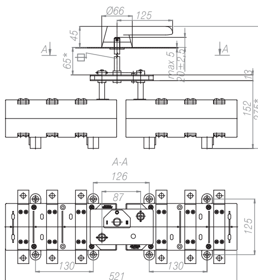
400 A – 630 A
